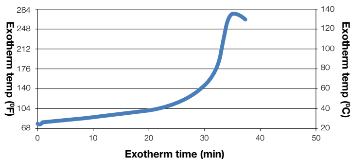
Typical Exotherm Curve for MA8120 (10g mass) 74°F (23°C) 5
