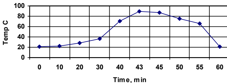
Typical Exotherm Curve for MA1025 at 23°C (10 grams) 5
